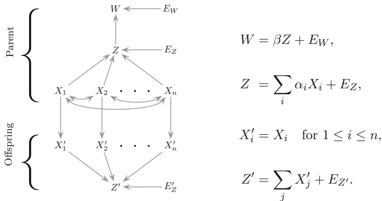
Fig. 1 A causal model underlying the breeder's equation. For the sake of simplicity the model here does not consider sexual reproduction or mutation. Double-edged arrows in the graph represent statistical dependence, or linkage disequilibrium, among parental genes. The structural equations on the right quantitatively specify each causal relationship in the graph
